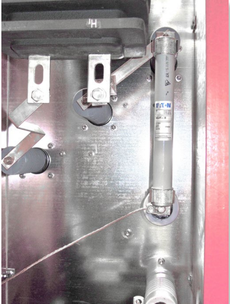
Optional C-H Type CLPT VT fuse - 15kV or 25kV - .5E A on (3) three bushings per phase units only
