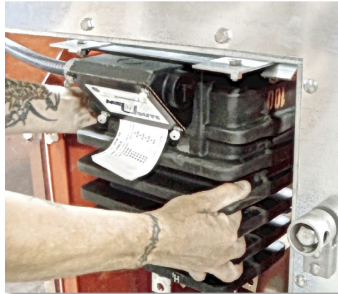
Slide-in CT stainless steel mounting hardware allows for ease of installation or removal
