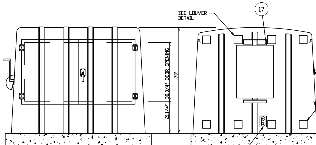
CABLE ENTRANCE COVER PLATE
