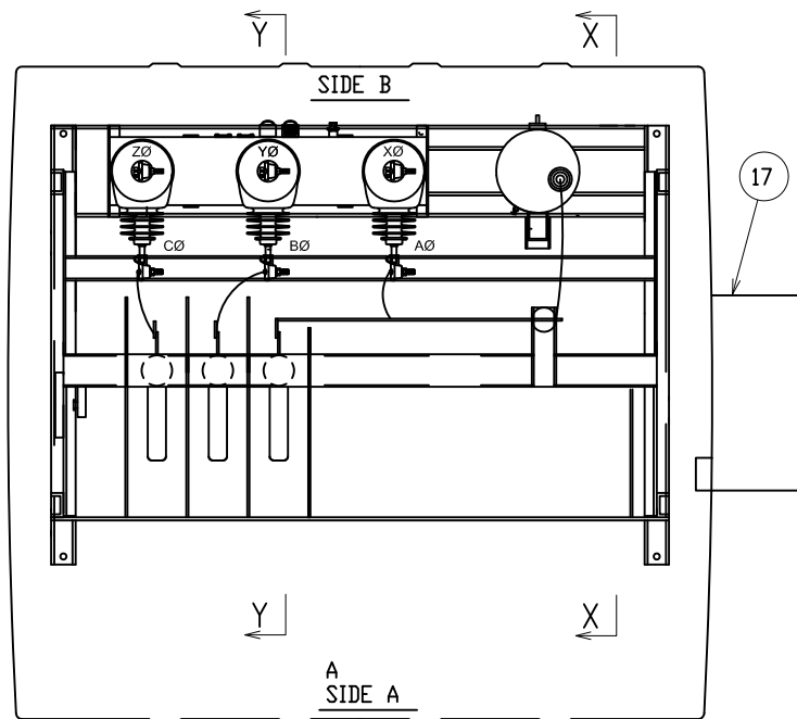
SECTION Z-Z
