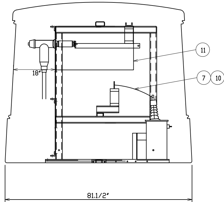
SECTION X-X
