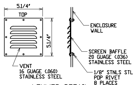
LOUVER DETAIL
