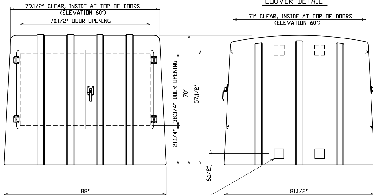
END VIEW
