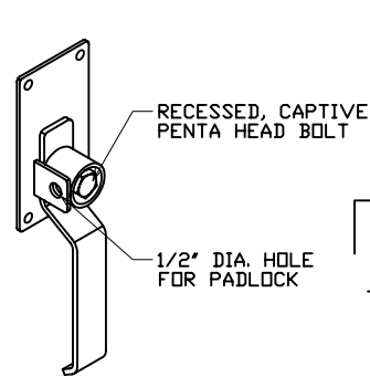
LATCH HANDLE DETAIL
