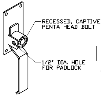
LATCH HANDLE DETAIL
