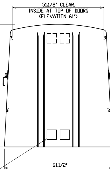
END VIEW
