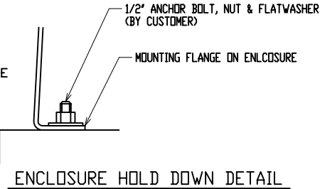
ENCLOSURE HOLD DOWN DETAIL
