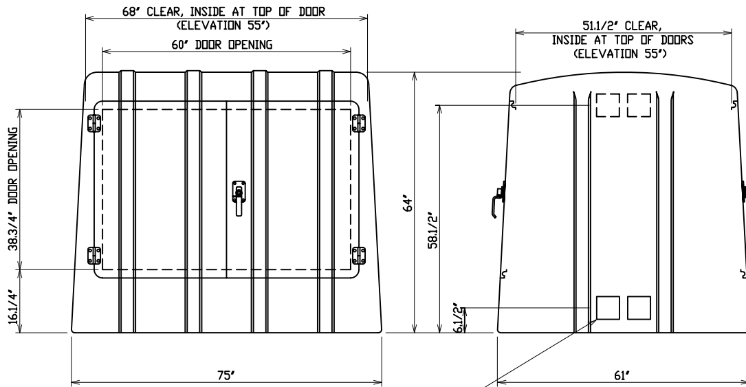
END VIEW
