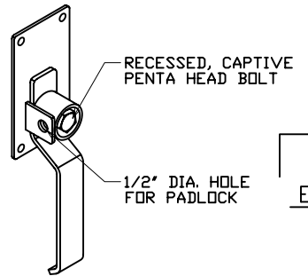
LATCH HANDLE DETAIL
