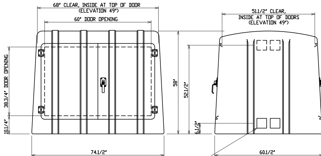
FRONT VIEW
