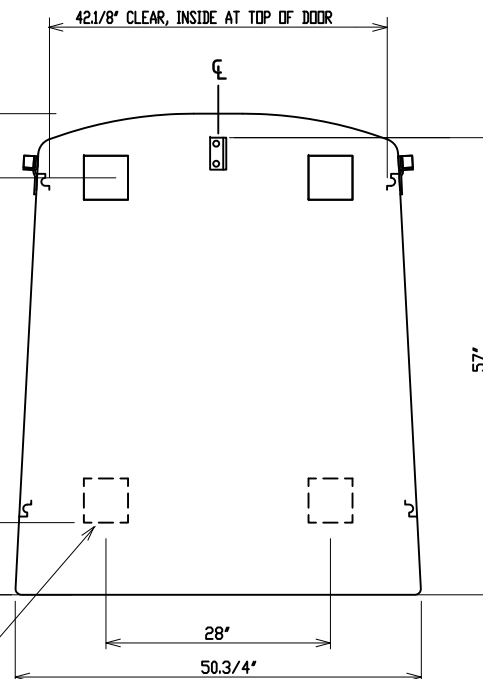
END VIEW
