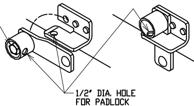
LATCH DETAIL
