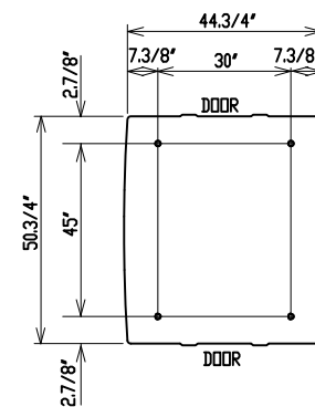
ANCHOR BOLT DIMENSIONS
