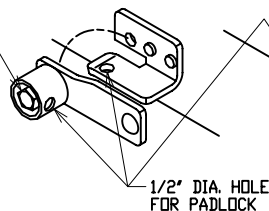
LATCH DETAIL
