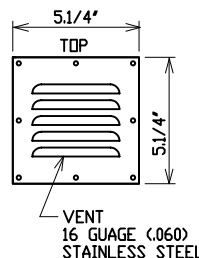
LOUVER DETAIL
