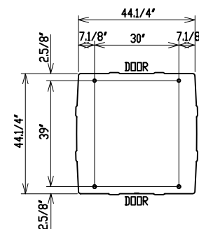
ANCHOR BOLT DIMENSIONS
