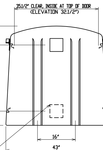
END VIEW
