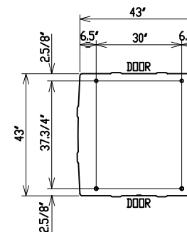
ANCHOR BOLT DIMENSIONS
