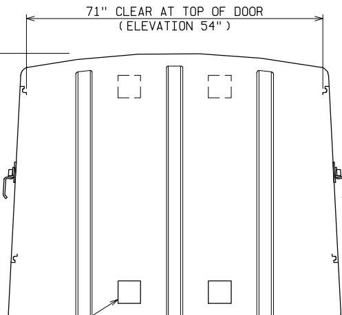
LOUVER DETAIL
