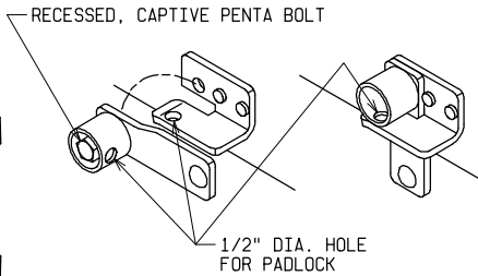
LATCH DETAIL
